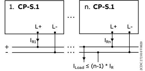
Parallel operation, redundancy ( n \leq 3 )
