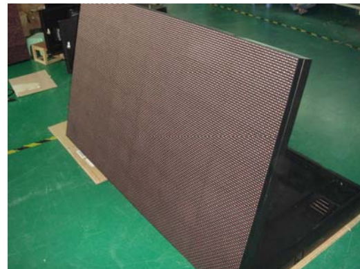
Front-Maintenance Cabinet Structure
