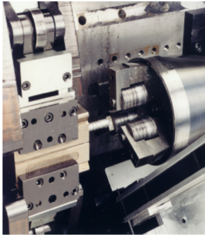
Servo Controlled Roll Groover, integrated or stand alone.
