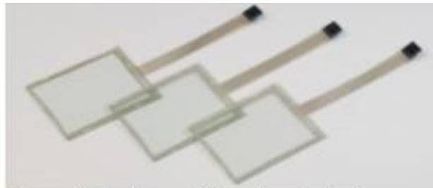
Glass with bus bar and flex wires attached
