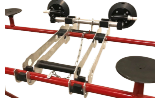
K4600-2-2 Glasstable with tilt function and vacuum suction cup ( for worktable )
